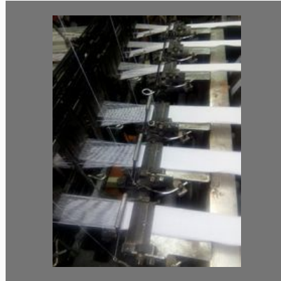
Cotton Belt Needle Loom Machine
